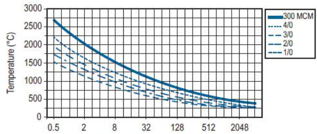
GPE320 Pulse Current Capability/脉冲电流
