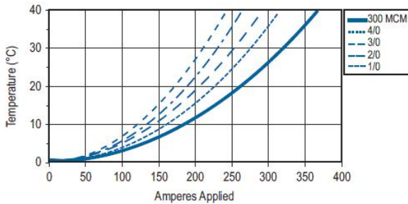
GPE320 Temperature Rise at Constant Current/温升曲线
